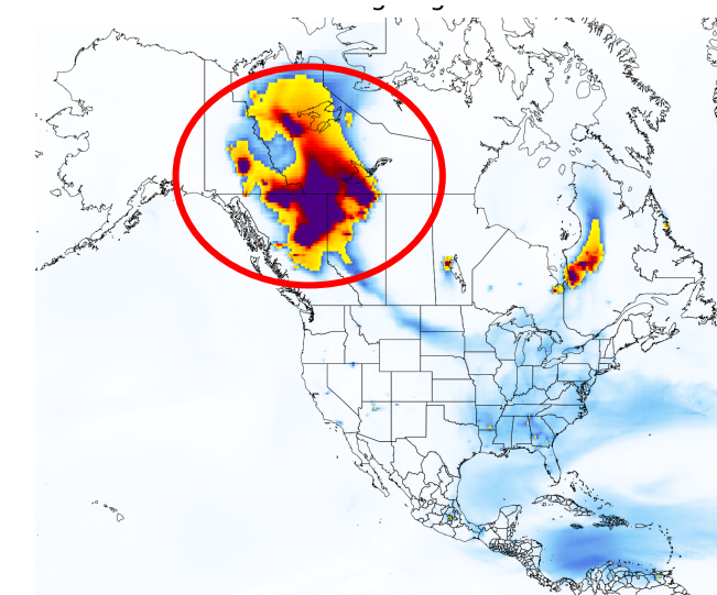
Ensemble Mean PM_{2.5}
