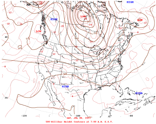
500 hPa Contours
