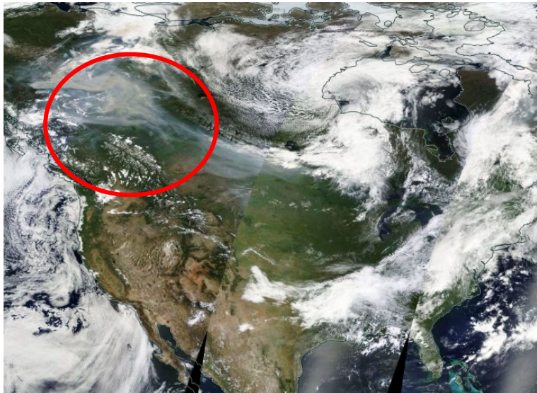
NOAA-20 True Color Image (July 9)
