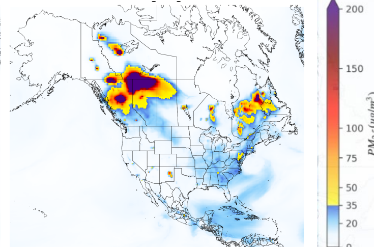
Ensemble Mean PM_{2.5}
