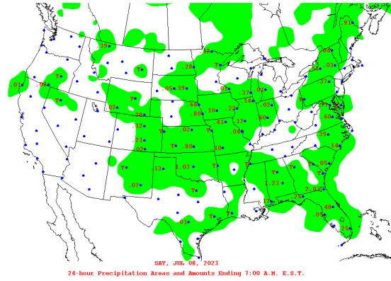
Precipitation
