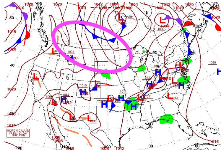
Surface Weather
