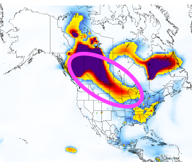
NAAPS \text{PM}_{2.5}
