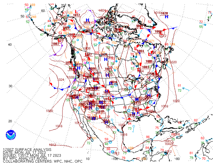
Surface Analysis
