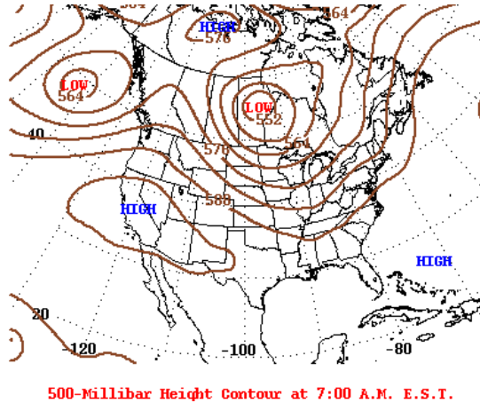
500 hPa Contours
