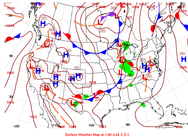
Surface Weather
