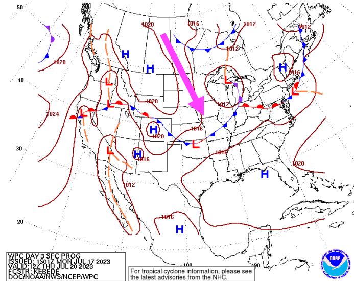
Sea Level
