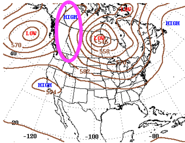
500 hPa Contours
