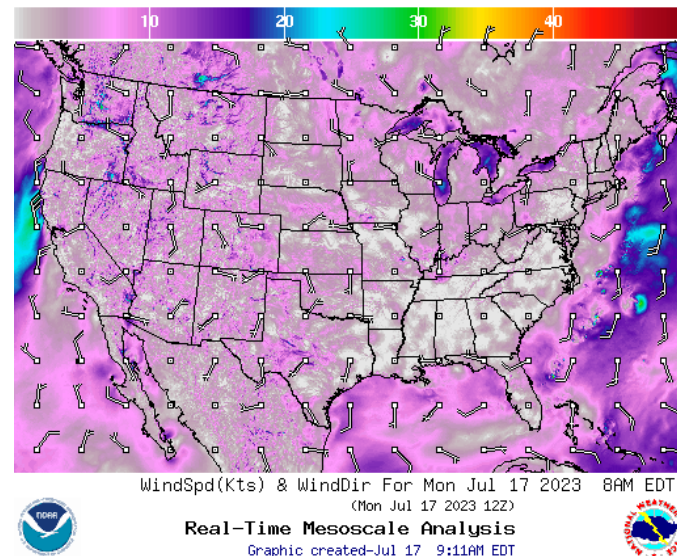
Wind Speed/Direction
