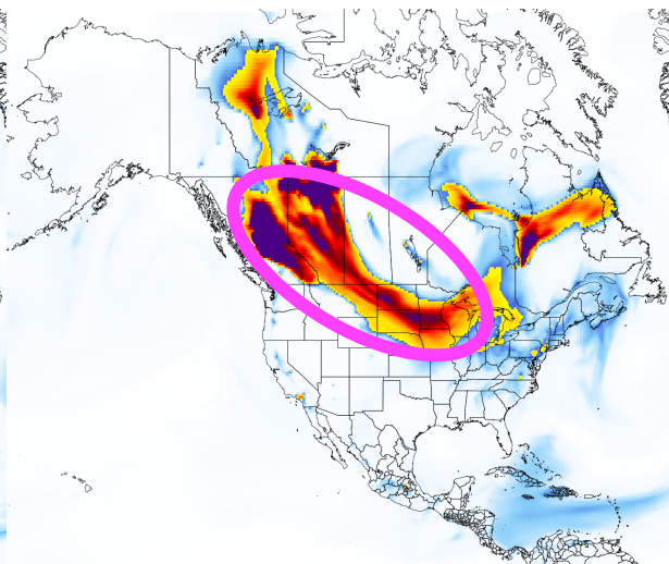
GEOS-CF \text{PM}_{2.5}
