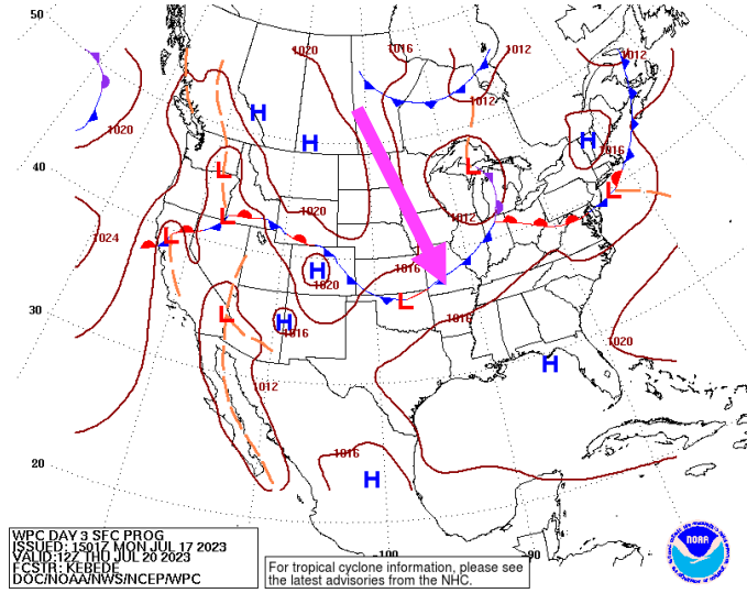
Sea Level
