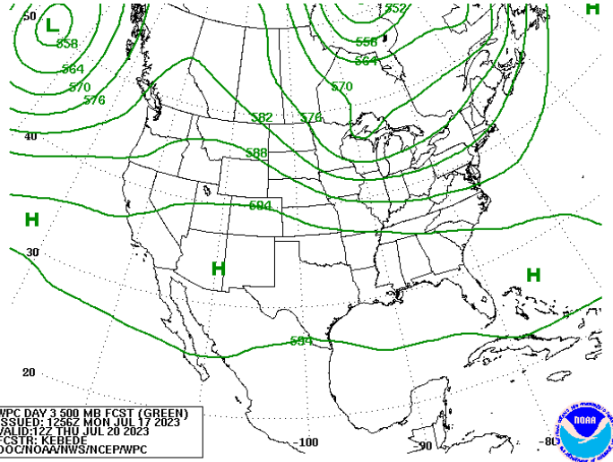
500 hPa Contours
