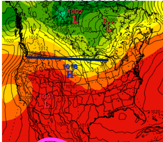
500 mb Contours
