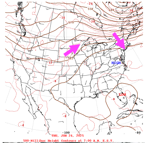
500 mb Contours
