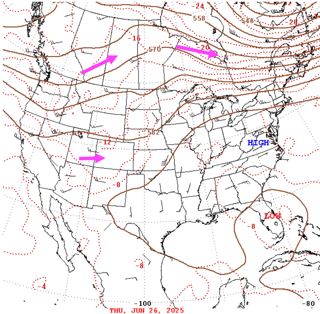
500 mb Contours
