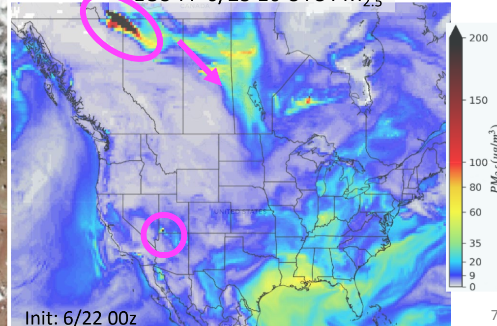
GEOS-FP 6/23 16 UTC PM 2.5
