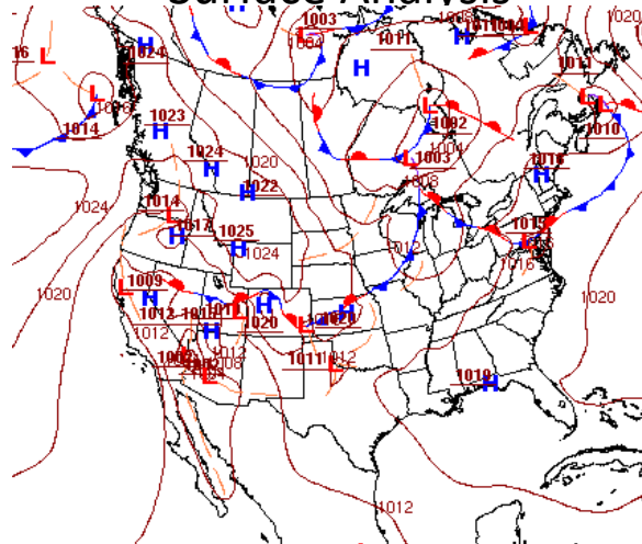
Surface Analysis
