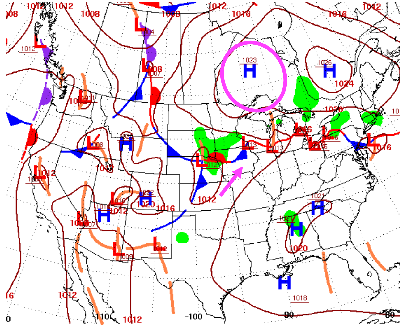
Surface Weather
