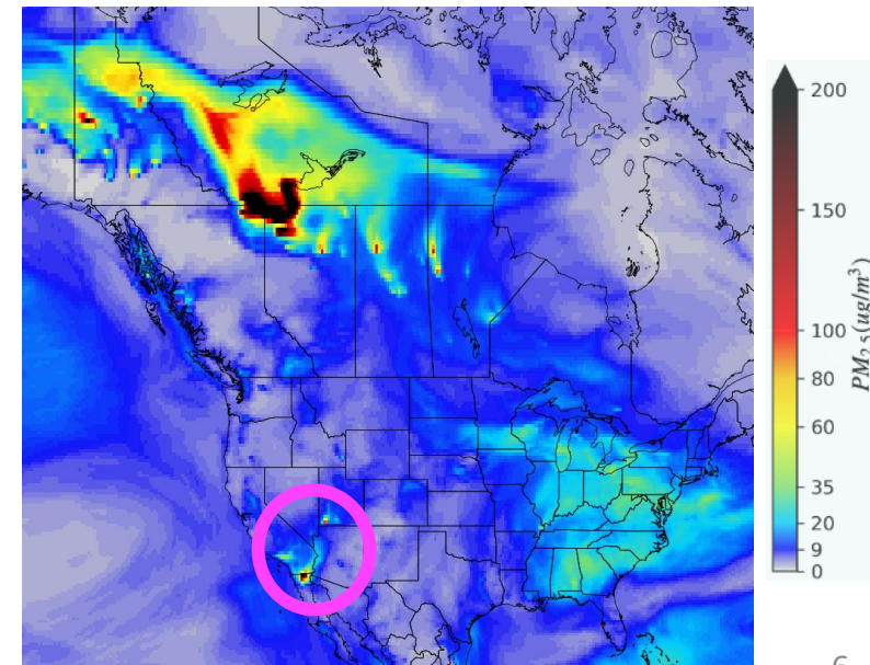
Ensemble
