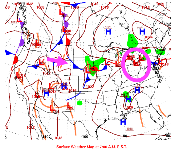
Surface Weather
