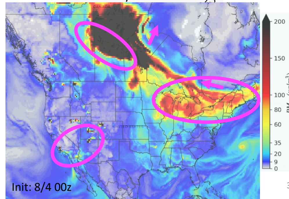
GEOS-FP 8/4 16 UTC PM 2.5
